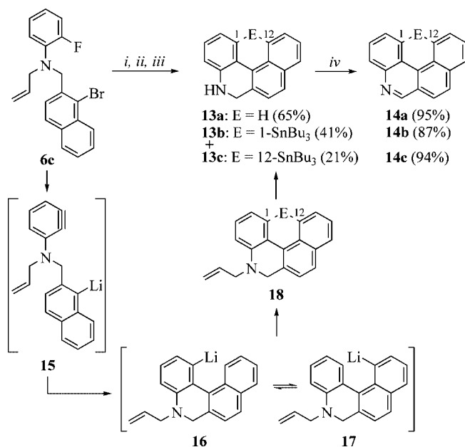
Scheme 5. Synthesis of dihydrobenzo[ k ]phenanthridines 13 and benzo[ k ]phenanthridines 14 ; reagents and conditions: i) t BuLi (3.5 equiv.), THF, –110 to 20 °C; ii) E + (1.5 equiv.), –78 to 20 °C; iii) DIBAL-H (1.5 equiv.), [NiCl 2 (dppp)] (4 mol-%), toluene, 20 °C; iv) PCC (1 equiv.), CH 2 Cl 2 , reflux.
