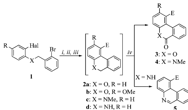
Scheme 2. Synthesis of dibenzo[ b,d ]pyran-6-ones 3 , phenanthridinones 4 , and phenanthridines 5 ; reagents and conditions: i ) t BuLi (3.3 equiv. for 1a,b , 3.5 equiv. for 1c,d ), THF, –110 to 20 °C; ii ) E + (1.5 equiv.), –78 to 20 °C; iii ) for 1d , DIBAL-H (1.5 equiv.), [NiCl 2 (dppp)] (4 mol-%), toluene, 20 °C; iv ) PCC (3 equiv. for 2a–c , 1 equiv. for 2d ), CH 2 Cl 2 , reflux.
