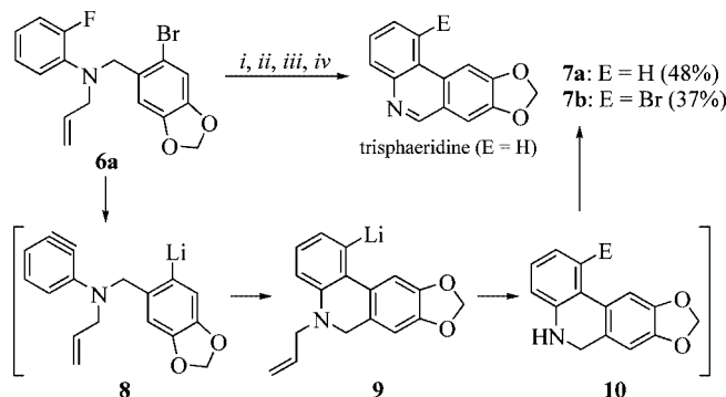
Scheme 3. Synthesis of trisphaeridine 7a ; reagents and conditions: i) t BuLi (3.5 equiv.), THF, -110 to 20\text{ }^{\circ}\text{C} ; ii) \text{E}^+ (MeOH, excess or \text{Br}(\text{CH}_2)_2\text{Br} , 1.5 equiv.), -78 to 20\text{ }^{\circ}\text{C} ; iii) DIBAL-H (1.5 equiv.), [\text{NiCl}_2(\text{dppp})] (4 mol-%), toluene, 20\text{ }^{\circ}\text{C} ; iv) PCC (1 equiv.), \text{CH}_2\text{Cl}_2 , reflux.
