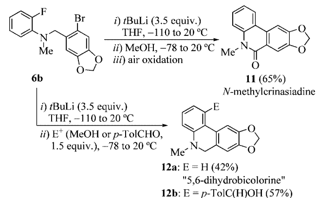
Scheme 4. Synthesis of N -methylecrinasiadine 11 and the putative structure of 5,6-dihydrobicolorine 12a .
